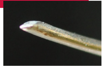
Regular "flipping" of the wheel results in self-sharpening of the wire tips for maximum performance.
